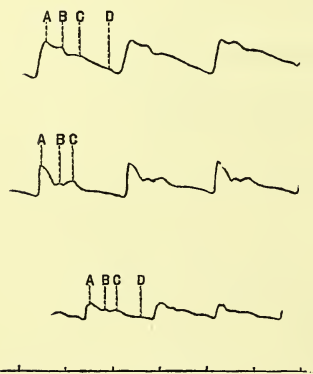
FIG. 47. PULSE TRACINGS FROM THE SAME RADIAL ARTERY UNDER DIFFERENT PRESSURES OF THE LEVER.
